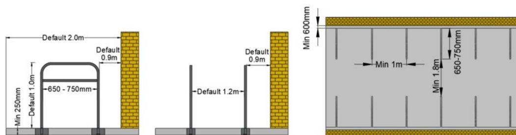
Figure 8: Typical Standard and Accessible Cycle Parking Arrangement
