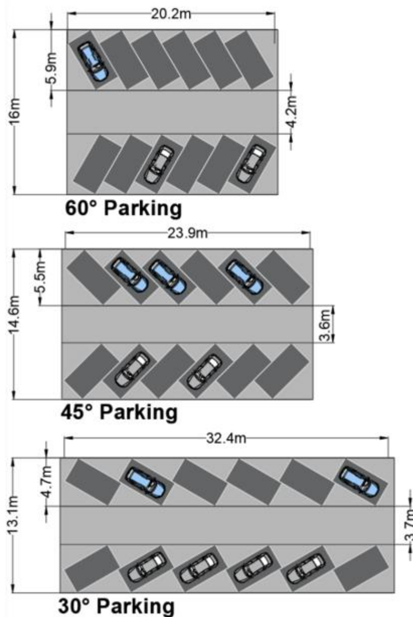
Figure 5: Angled Parking Arrangement
