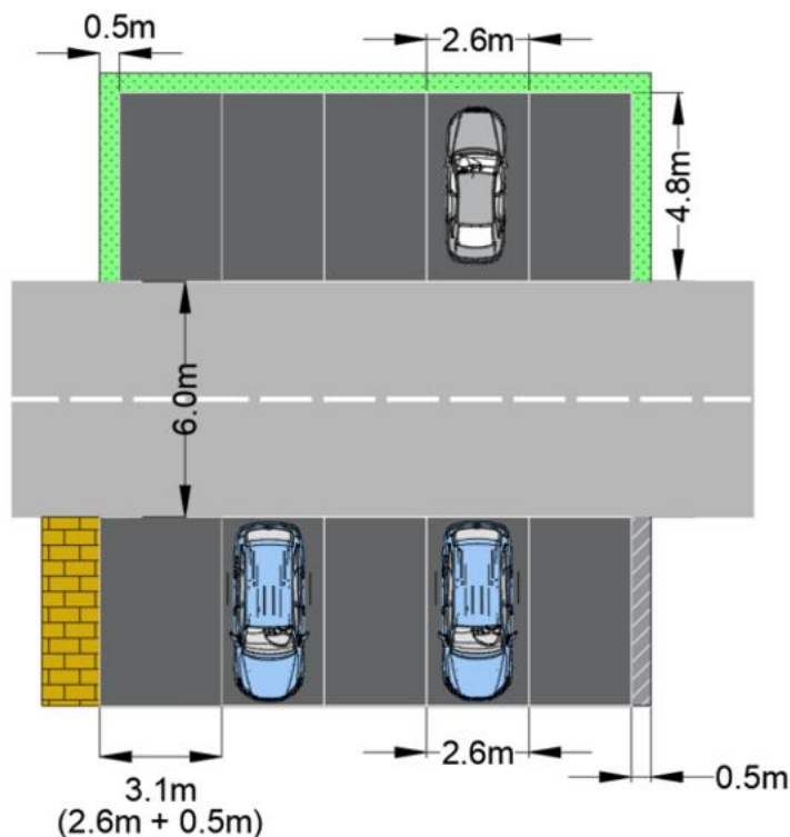
Figure 3: Perpendicular Parking Arrangement
