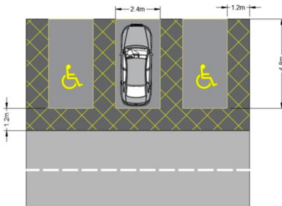
Figure 7: Disabled Parking Arrangement
