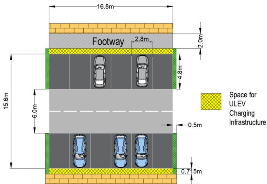
Figure 9: Electric Vehicle Parking Arrangement
